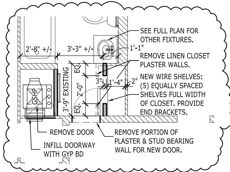
3 LINEN CLOSET DETAIL PLAN A304 SCALE: 1/4" = 1'-0"
