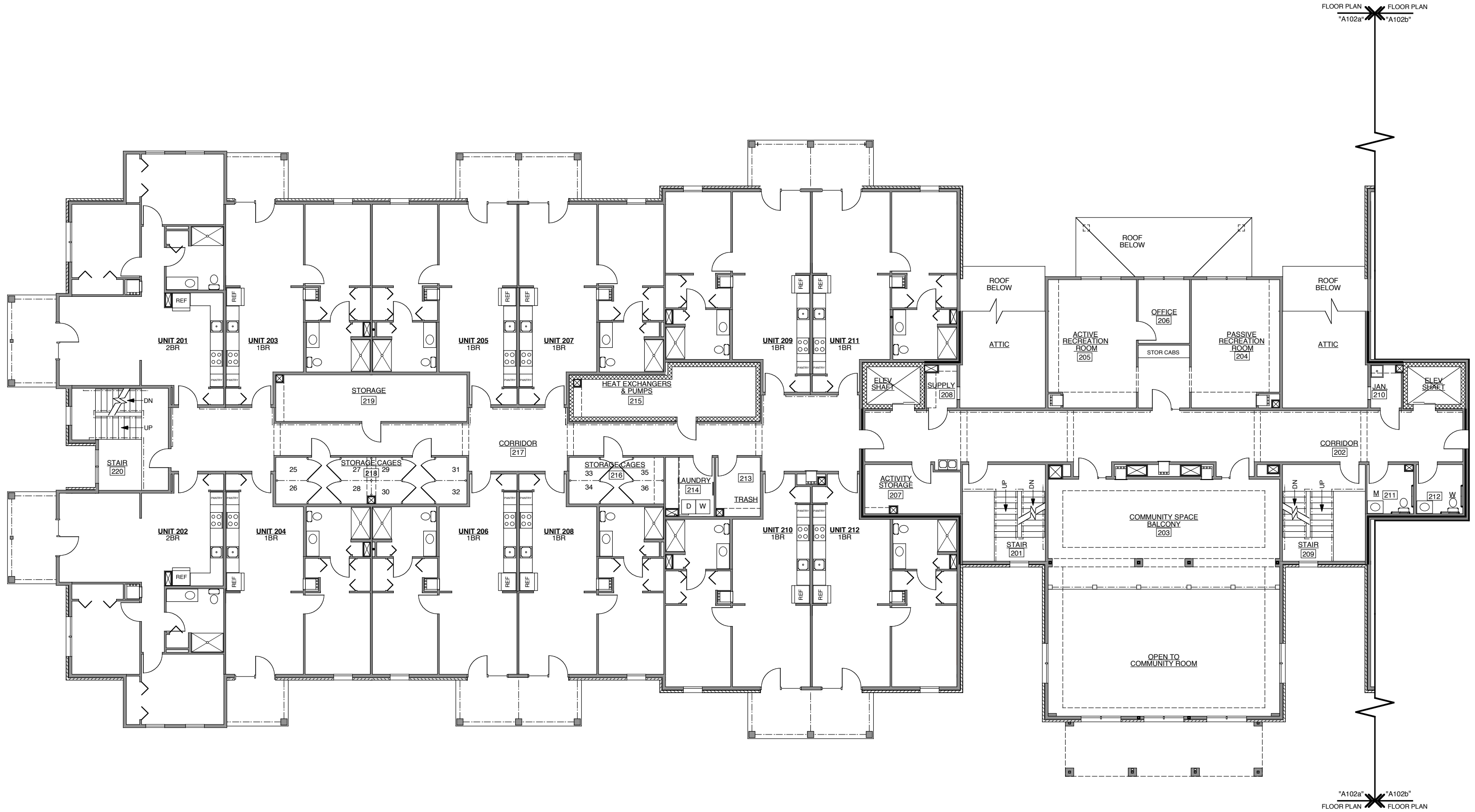
1 SECOND FLOOR PLAN "a" A102a SCALE: 1/8" = 1'-0"
